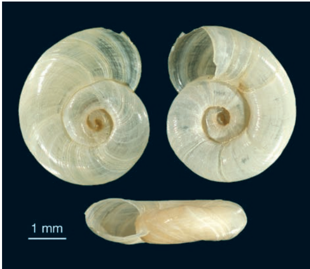
Abb. 4. Gyraulus ehrenbergi (Topotypus, ex coll. Meier-Brook).
