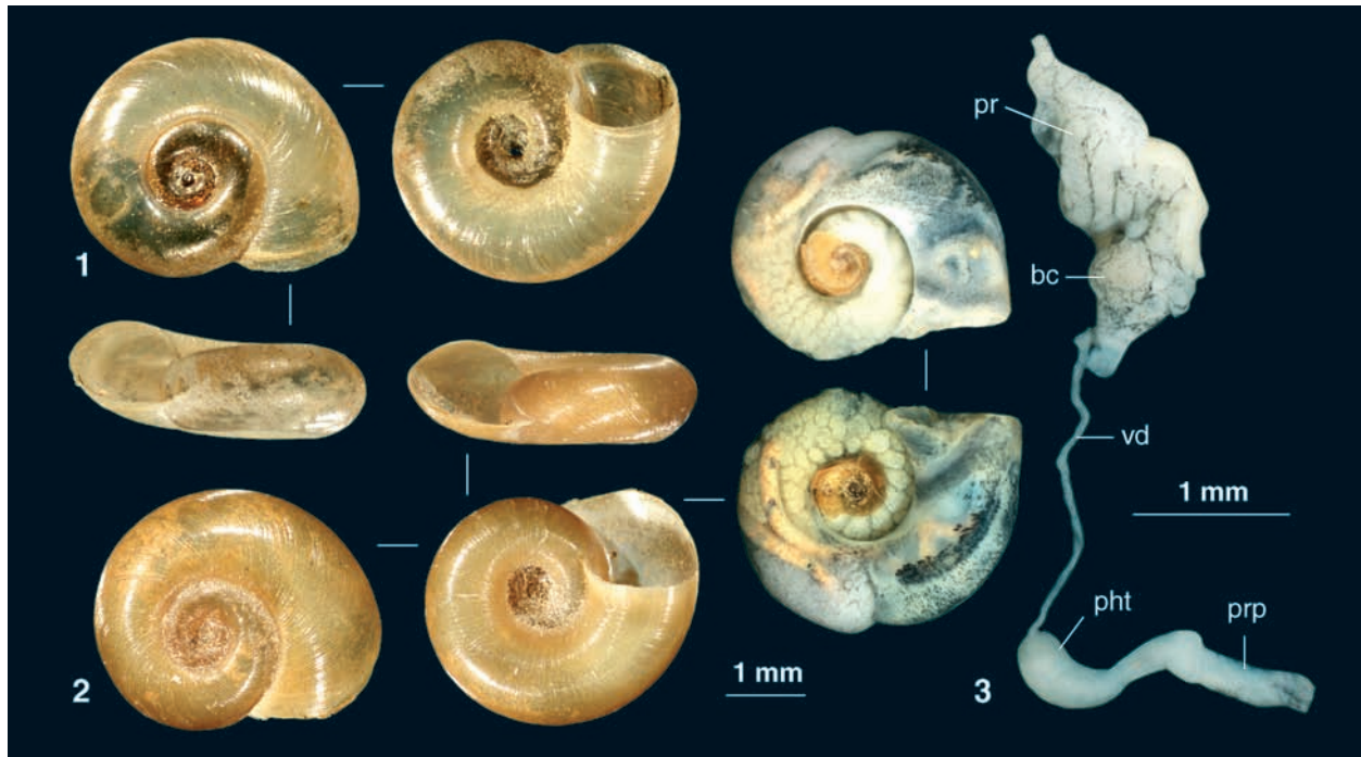
Abb. 3. Gyraulus piscinarum . 1: Paratypus, 2: Topotypus, 3: Genitaltrakt. – bc = Bursa copulatrix, pht = Phallosome, prp = Praeputium, pr = Prostata.
