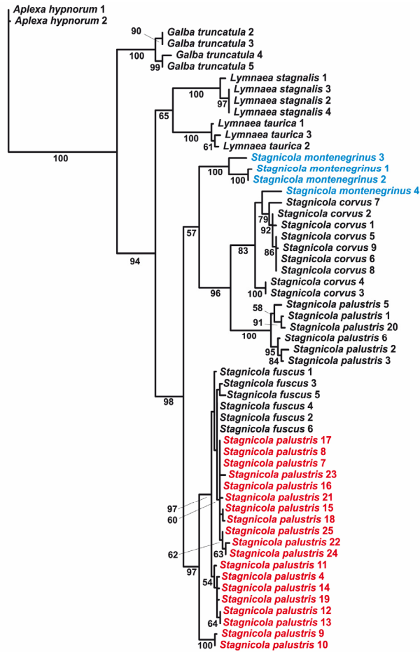
Figure 3. Hypothesis of the phylogenetic relationships of Stagnicola : Best maximum-parsimony tree of the fragment sequenced of the mitochondrial marker cyt-b (329 bp). Branch lengths are proportional to the number of substitutions. Bootstrap support values above 50% are reported below nodes. Hybrids between S. palustris and S. fuscus are marked red. Specimens of S. montenegrinus are marked blue.
